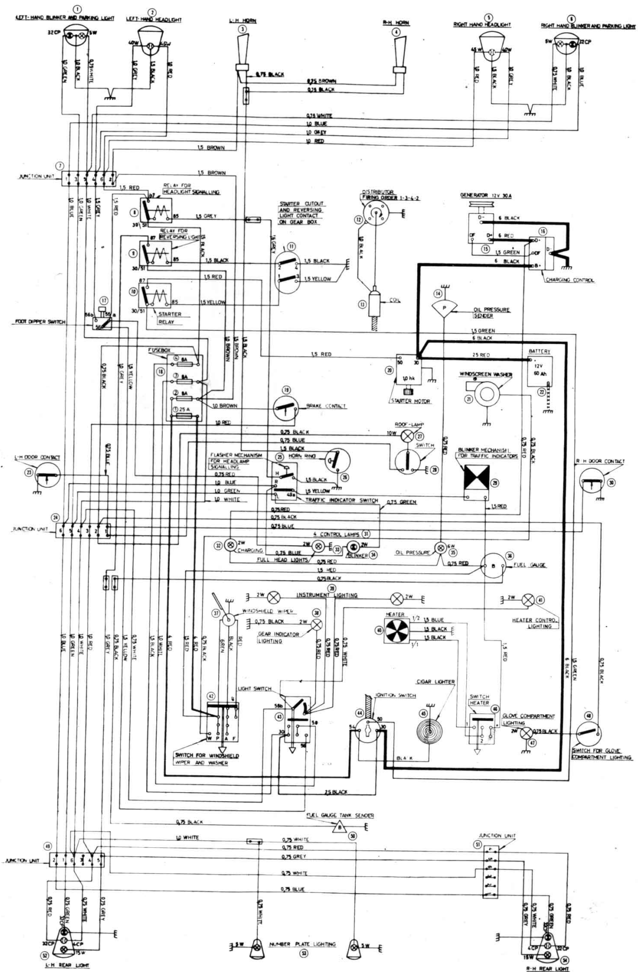
120 Series Saloon with automatic transmission
